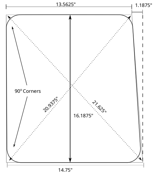
Window D Fixed Thickness: 3/8" Qty: 2 One port One starboard 3" radius
