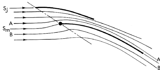
Figure 2. Typical wrong slot-effect drawing.
